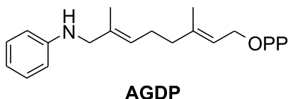
Fig. 5. The AGDP analogue described by Spielmann [16].
