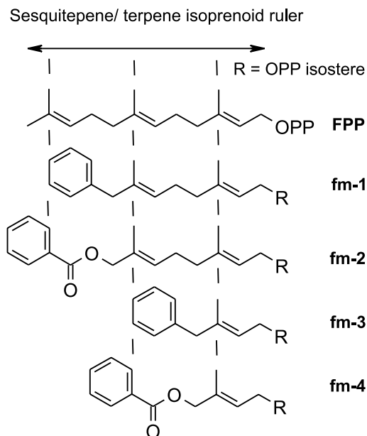
Fig. 1. Molecular ruler hypothesis for isoprenoid specificity.
