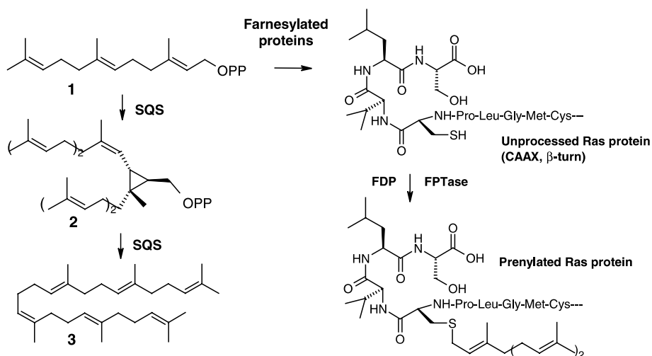
Scheme 1. FDP ( 1 ) is converted into squalene ( 3 ) by SQS and utilised by FPTase in the S-prenylation process.
